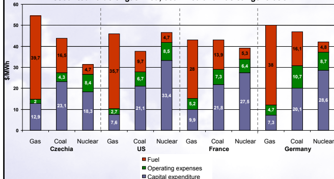
Discounted value of gas-fired, coal-fired and nuclear generation
